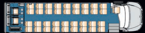
36 Passenger Plus 2 Wheelchair 2 Passenger Foldaway and 4 Passenger Flip Seats Plus Driver
