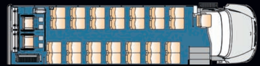
28 Passenger Plus 2 Wheelchair 2 Passenger Foldaway and 4 Passenger Flip Seats Plus Driver
